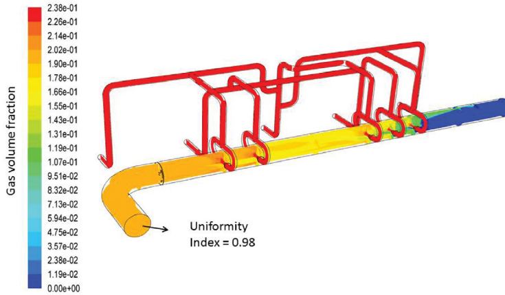
Figure 1. Contours of gas dispersion across representative cross-sectional planes, Case 1
