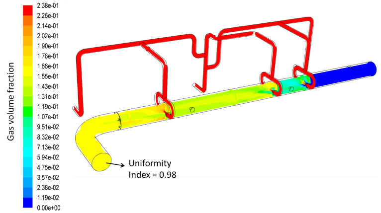
Figure 2. Contours of gas dispersion across representative cross-sectional planes, Case 2
